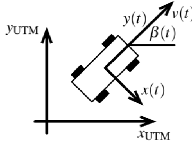
Fig. 1. State values representing the process model.
