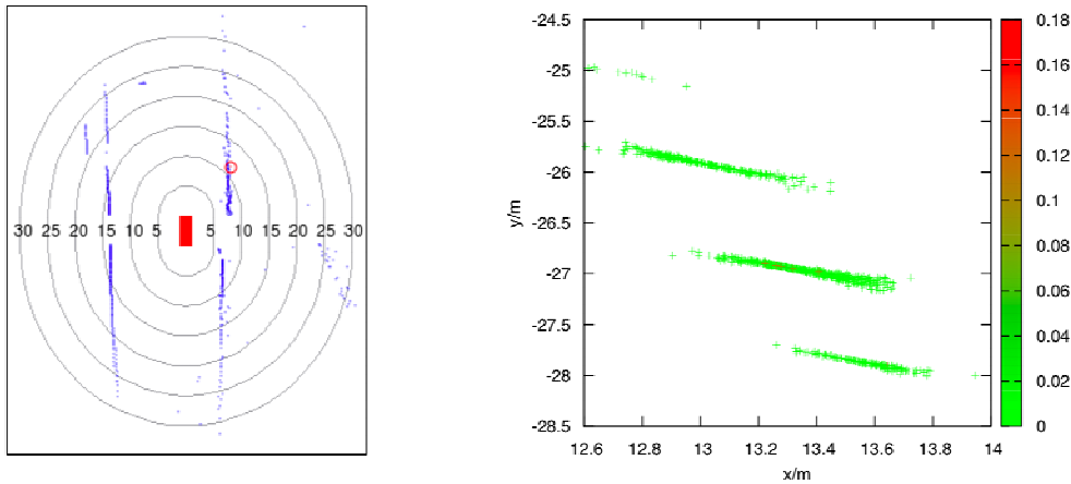
Fig. 5. State distribution of a street surrounded by natural objects.
