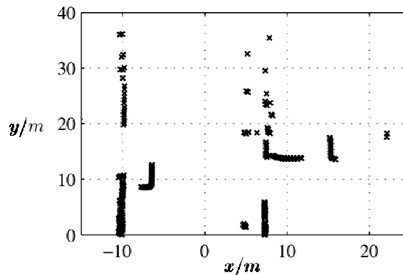
Fig. 2. Raw data of a lidar scan.
